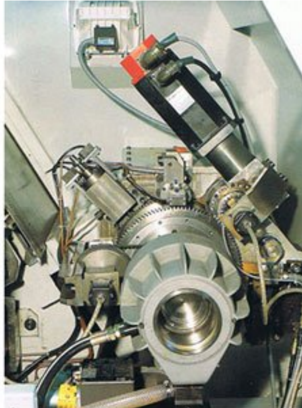
Third interpolated spindle axis (C axis) and dividing brake unit with spindle indexing
