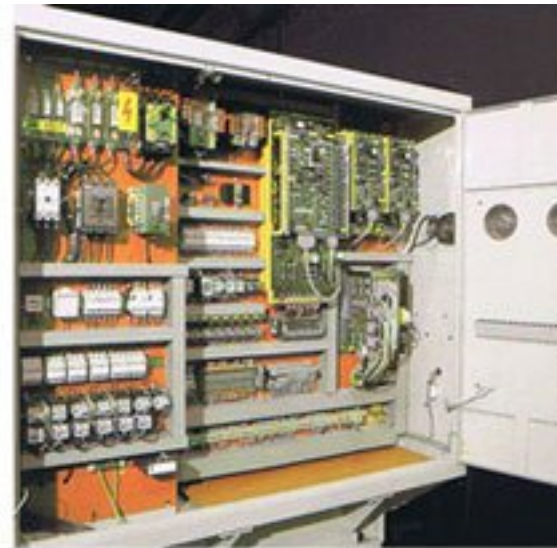
Inside of electric panel equipped with heat exchanger
