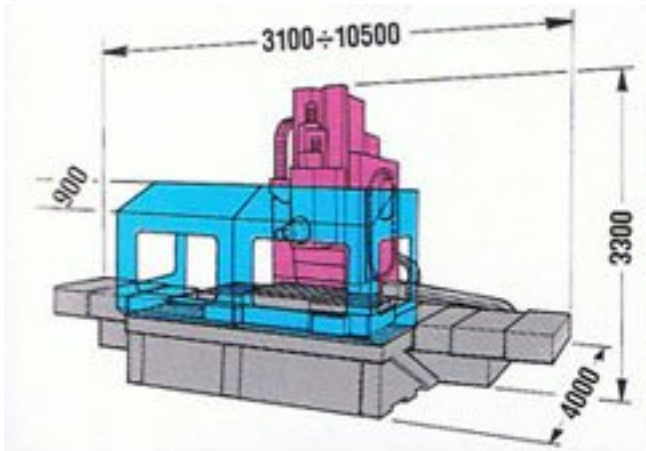
Chain tool change and cross movement
